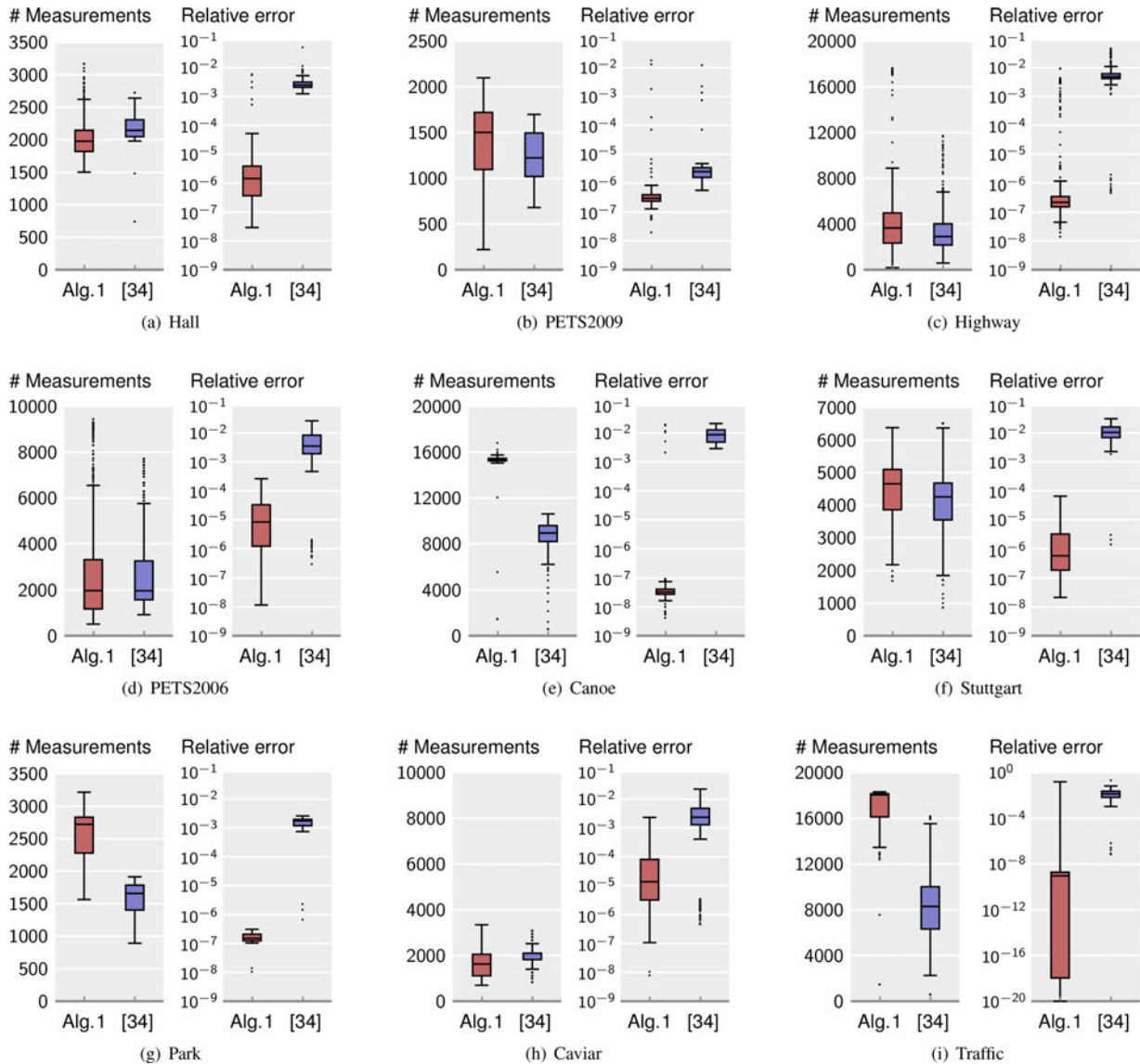
Fig. 4. Results of Type II experiments. Each subfigure corresponds to a line of Table I and contains two boxplots: one for the number of measurements and another for the reconstruction error. In a boxplot, the horizontal line is the median, the box extremes are the Q_1 and Q_3 quartiles, and the whiskers are the minimum and maximum of data that is within 3/2 of the interquartile range of Q_1 and Q_3 ; points outside this range (outliers) are represented with dots. (a) Hall, (b) PETS2009, (c) Highway, (d) PETS2006, (e) Canoe, (f) Stuttgart, (g) Park, (h) Caviar, and (i) Traffic.
