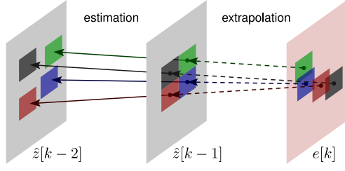
Fig. 2. Scheme of motion-compensated extrapolation. We use the motion between matching blocks in \hat{z}[k-2] and \hat{z}[k-1] to create an estimate e[k] of frame z[k] .
