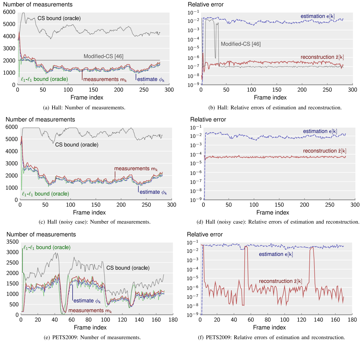
Fig. 3. Results of Type I experiments. The left-hand side plots show the number of measurements m_k taken from each frame (solid red line), the estimate \phi_k (dashed blue line), and the right-hand side of (7) and (8) (dotted green and black lines, respectively). The right-hand plots side show the relative errors of estimation \|e[k] - z[k]\|_2 / \|z[k]\|_2 and reconstruction \|\hat{z}[k] - z[k]\|_2 / \|z[k]\|_2 . (a) and (b) Hall sequence with noiseless acquisition; (c) and (d) Hall sequence with noisy acquisition; (e) and (f) PETS2009 sequence with noiseless acquisition.
