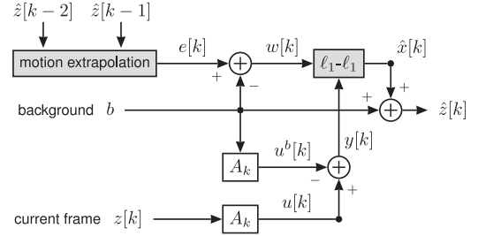
Fig. 1. Block diagram of Algorithm 1 when applied to background subtraction. The main blocks are highlighted.
